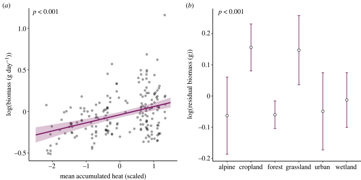
Figure 2. The effect of climate and habitat on total insect biomass in Sweden during 2019. Effect of (a) mean accumulated heat on the yearly total insect biomass, and (b) habitat types on the residual variation in biomass after accounting for the effect of accumulated heat. In (a), the solid trendline presents the significant relationship predicted by the model. In (b), circles represent estimated means with confidence intervals in purple for each habitat type as based on model predictions. The p -values of predictors are presented in the upper left corners. For model output related to this figure, including p -values, F -values and degrees of freedom, see electronic supplementary material, table S5a.
