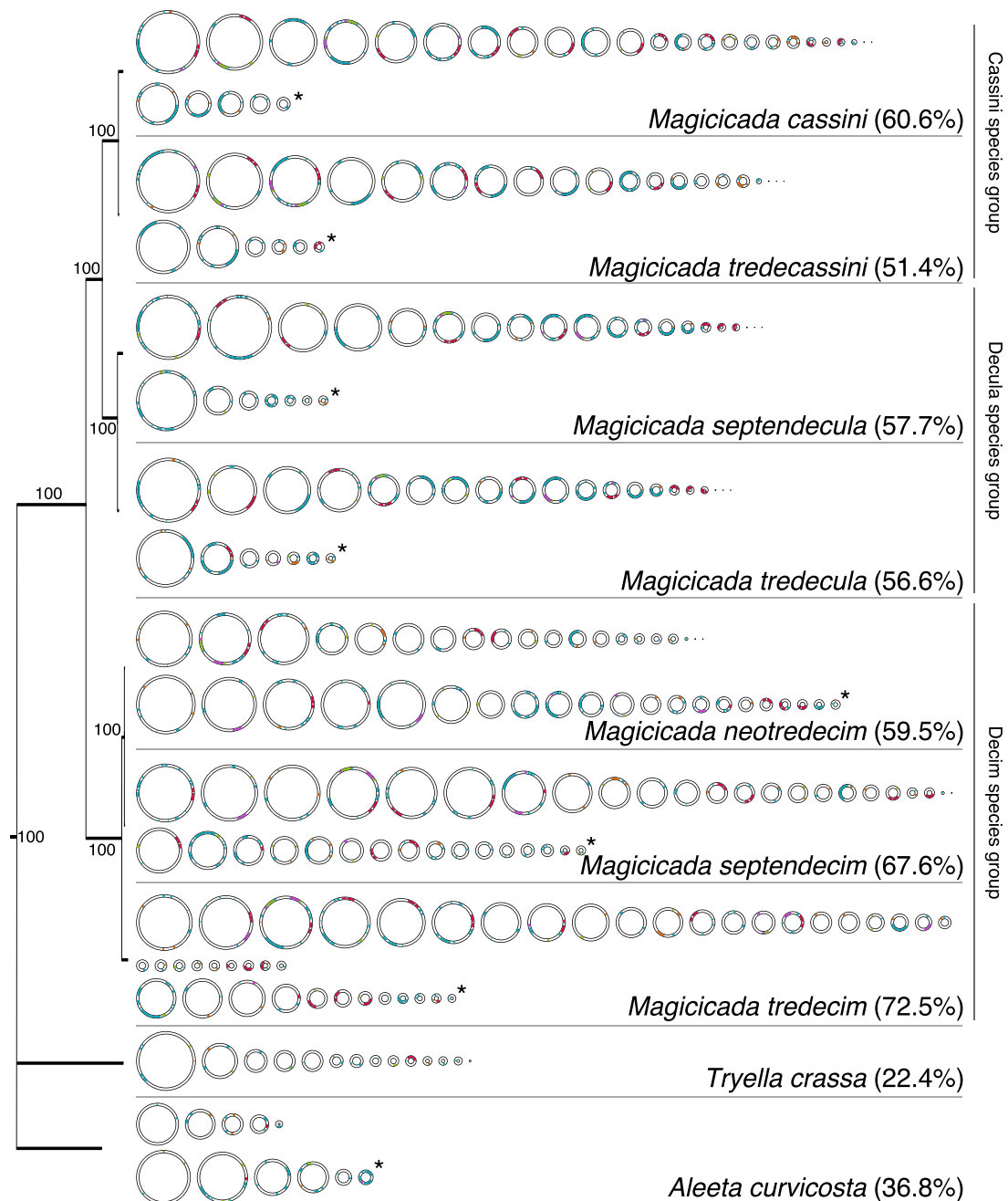
Figure 1. Hodgkinia Genomic Complexity in All Study Species
